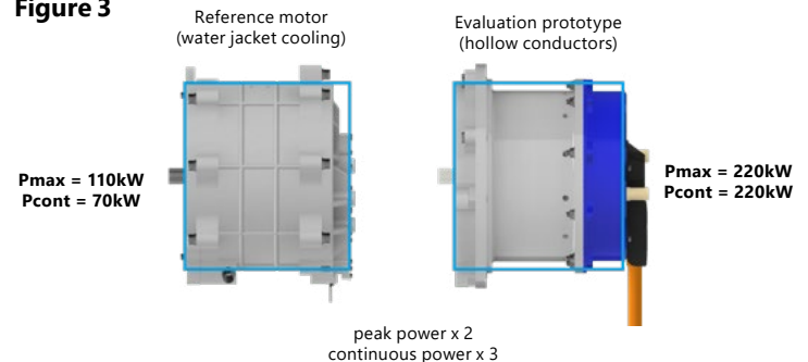
Figure 3. Comparison of peak and continuous power between an indirect and a direct-cooled electric motor. Source: Hyperdrives GmbH
