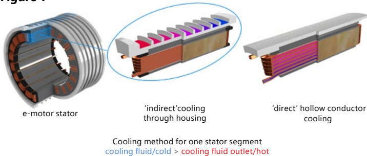
Figure 1. Exemplary stator segment to visualize the general concept of state-of-art indirect cooling and the innovation of direct cooling through hollow conductors. Source: Hyperdrives GmbH.
